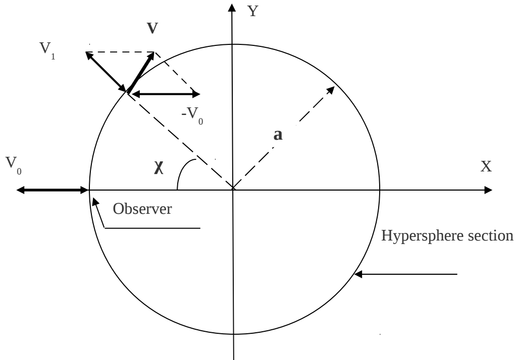
Picture 1. Two-dimensional section of the 4-dimensional Euclidean space with hypersphere of the radius «a». Angular coordinate \chi characterize the hypersurface point moving away from the observer (black spot). Vectors V_0 and V_1 - velocities of the movement of the observer and observed data. Vector V — velocity of the movement of the object in relation to the observer.
