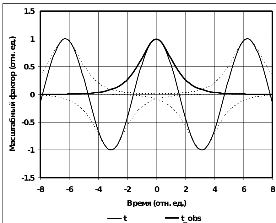
Picture 3. Dynamics of the development of the modified model of the Universe on the time scales of the hypersphere center ( t ) and observer in a 3-dimensional world ( t_{obs} ). Harmonic oscillations in the mass center system giving birth to the eternal Universes on every half-period of the oscillations.
