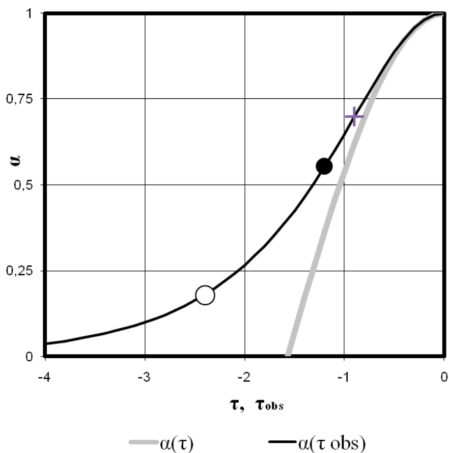
Picture 2. Dynamics of the expansion of the closed Universe with consideration of the dependency of the scale factor from time ( g_{00} = \gamma^{-2} ) in different coordinates. Time is expressed in relative units \tau \equiv (c/2a_0)t and is counted from the moment of the maximal expansion ( \alpha = 1 ). On the curvature \alpha(\tau_{\text{obs}}) we mark the positions of the current condition of the Universe at \Omega=0,03 (light circle) and at \Omega=0,4 (dark circle). The point of bend is marked with the cross.
