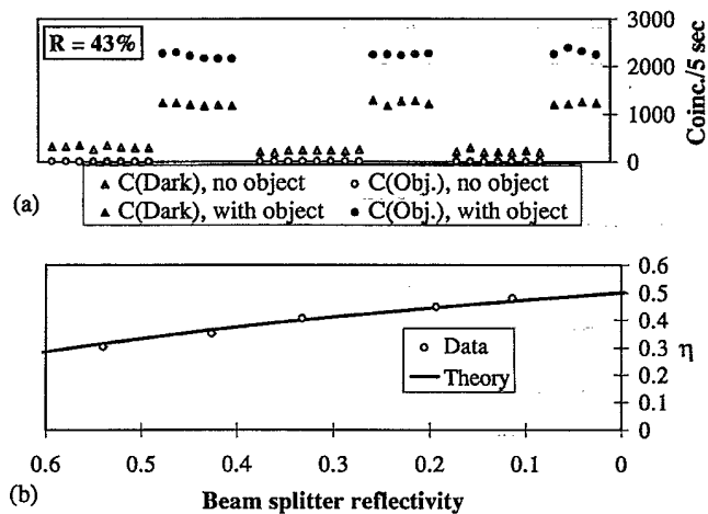
FIG. 5. (a) Typical experimental results for an interaction-free measurement. The beam splitter reflectivity for this data set was 43%. (b) Experimental and theoretical values for the figure of merit \eta in the Michelson-interferometer scheme, as a function of beam splitter reflectivity.
