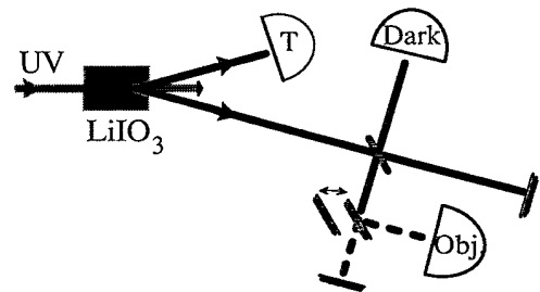
FIG. 4. Schematic of the down-conversion experiment demonstrating the principle of an interaction-free measurement.
